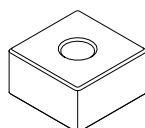
M6 20mm x 20 mm x 11mm Channel Nut
